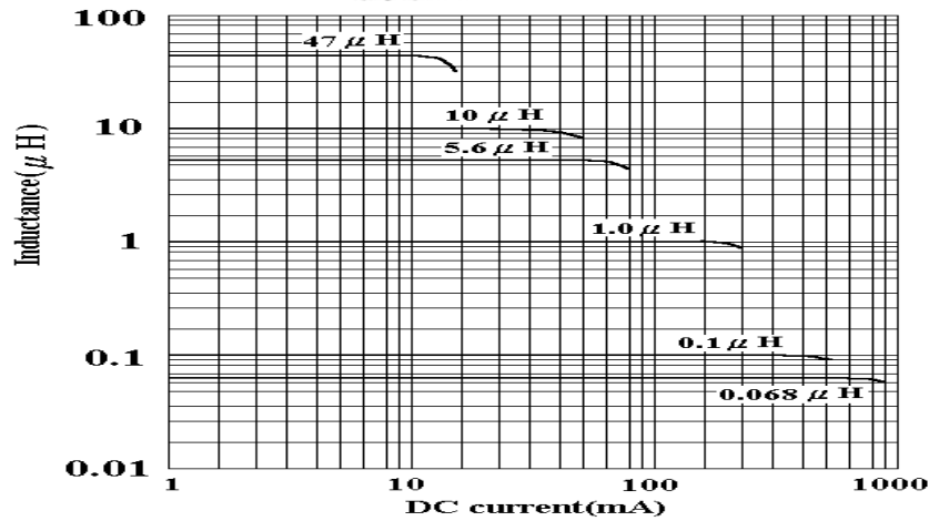
Inductance Vs. DC Superposition
