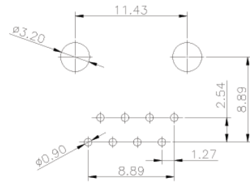
8P8C PC BOARD LAYOUT
