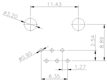
6P6C PC BOARD LAYOUT
