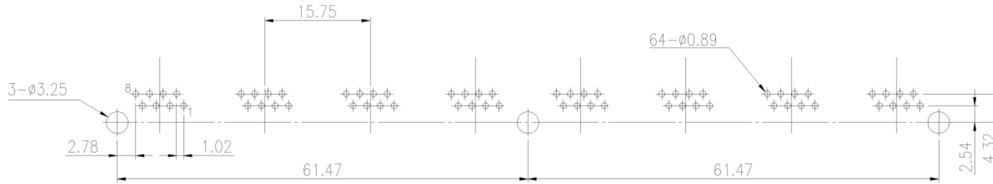
RECOMMENDED P.C.B. LAYOUT
