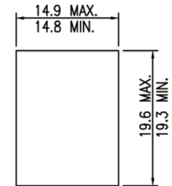
SINGLE PANEL-LATCH CLEARANCE PANEL THICKNESS 0.062 INCH
